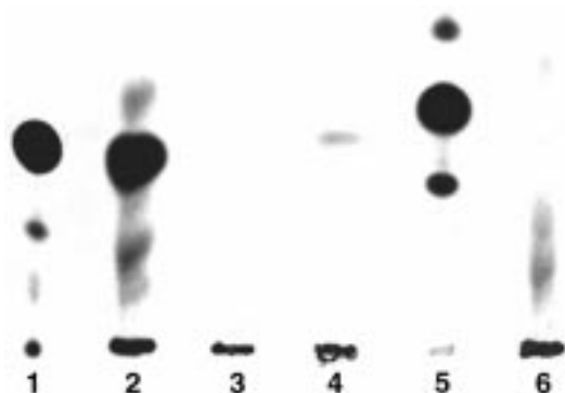
Figure 2. Autoradiogram of thin layer chromatogram of ^{14}\text{C} -labeled BABA and ^{14}\text{C} -labeled GABA treated Arabidopsis . Lane 1: ^{14}\text{C} -labeled BABA; lane 2: ground whole protoplasts of a ^{14}\text{C} -labeled BABA treated plant; lane 3: cell wall fraction of a ^{14}\text{C} -labeled BABA treated plant; lane 4: membrane and organelle fraction of a ^{14}\text{C} -labeled BABA treated plant; lane 5: ^{14}\text{C} -labeled GABA; lane 6: ground whole protoplasts of a ^{14}\text{C} -labeled GABA treated plant. Protoplast were isolated and ground directly in microtubes, the debris spun down and the supernatant (cell contents) applied to TLC plates. The pellet was washed four times with MCW (MeOH: \text{CHCl}_3 : water 12:5:3 (v/v)) to yield the membrane fraction. The cell wall fraction was obtained by spinning down the remains in the protoplasting enzyme solution after the protoplasts had been released and washing them four times in MCW. TLC plates were run in a solution of n-butanol: HAC: water 60:20:20 (v/v).
